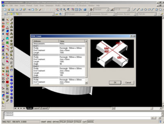
Figure 3: HVAC fully supports both on-the-fly and catalog based modeling
