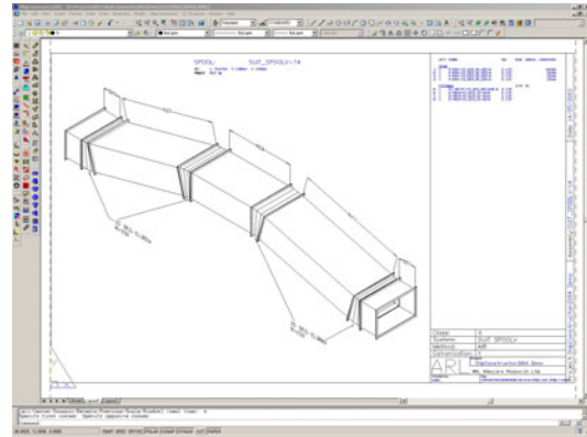
Figure 5: Automatic generated Spool Isometric Drawings
