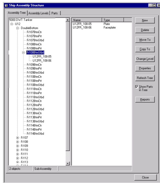
Figure 2 –Part Tree
