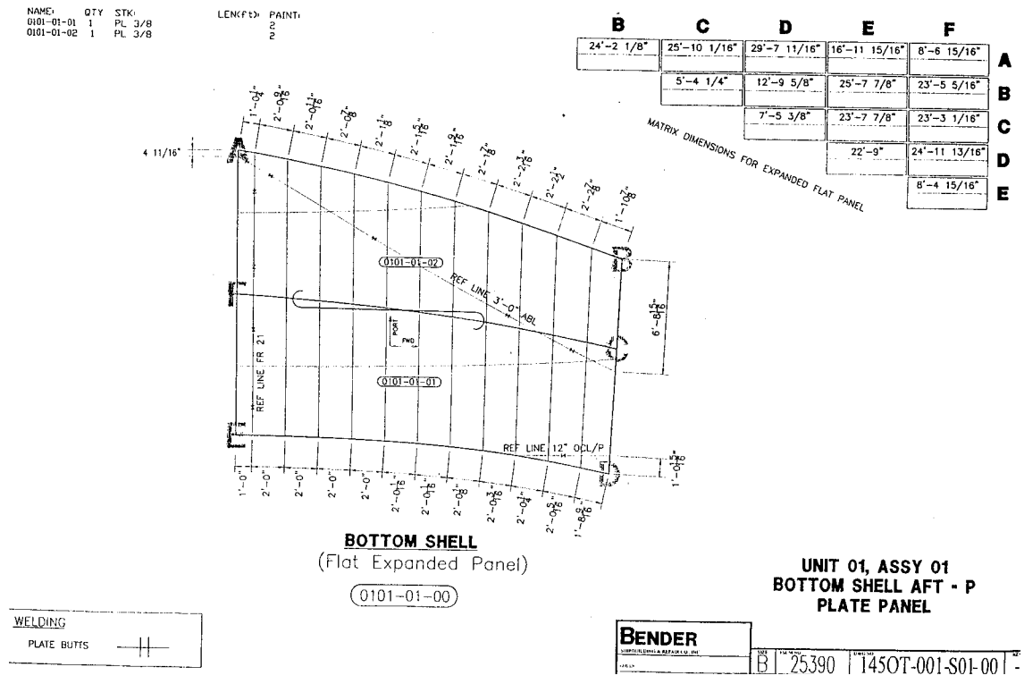
Figure 1 - Work Sketch
